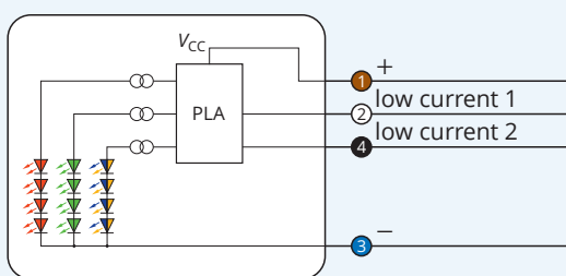
Pinout
