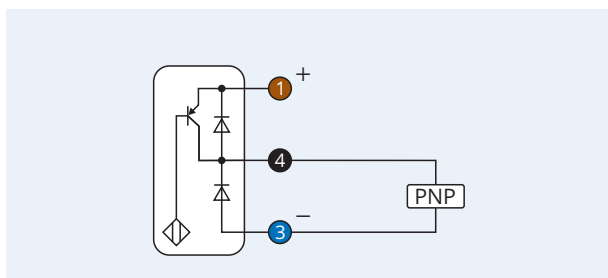
Pinout
