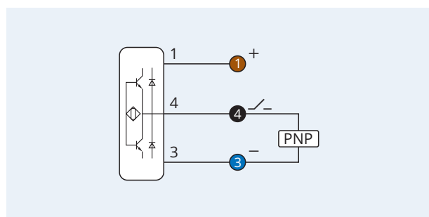
Pinout
